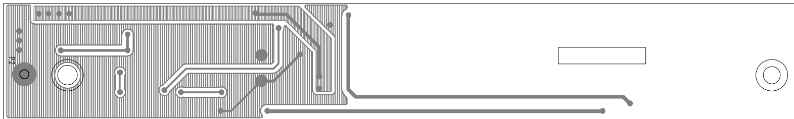
9.0 COMPONENT LAYOUT DVD1650H HV PCB BOARD DIAGRAM
